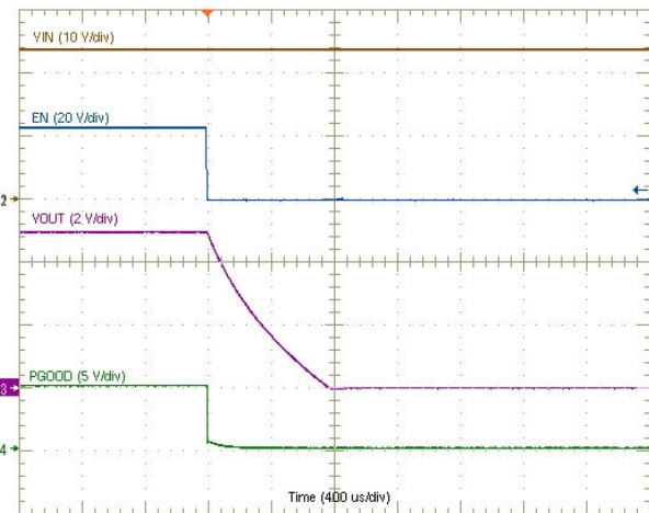
Figure 8-3. Enable Shutdown Waveforms
