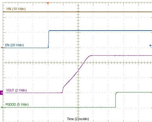
Figure 8-2. Start-Up Waveforms
