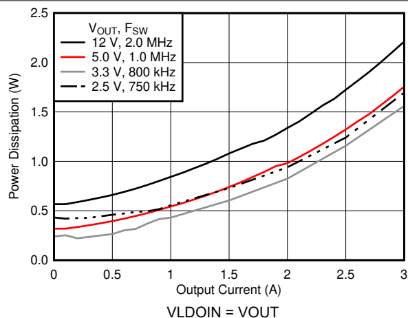
Figure 6-14. Power Dissipation
