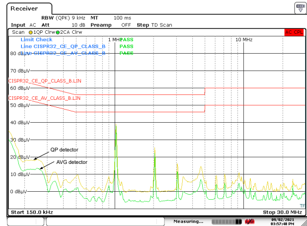
Figure 9-9. CISPR 32 Class B Conducted Emissions: V_{IN} = 24 V
