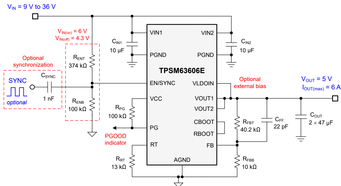
Figure 9-1. Circuit Schematic
