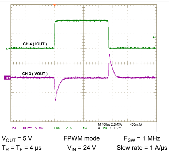
Figure 9-7. Load Transient, 0 A to 4 A, 1 A/ \mu\text{s}
