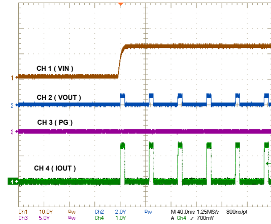
Figure 9-9. Start-up into Short Circuit
