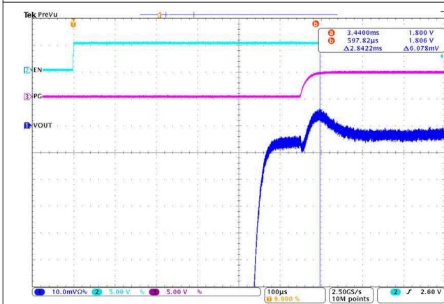
Figure 8-48. HICCUP Short-Circuit Protection (Zoom In)
