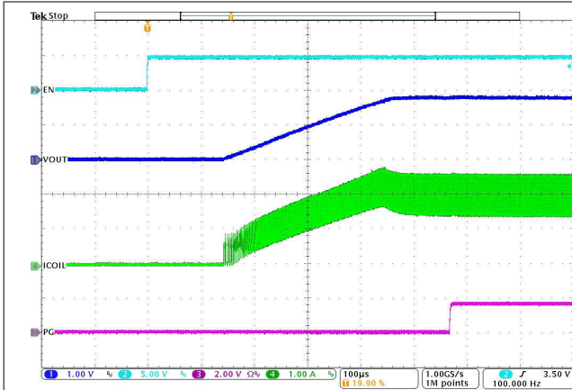
I_{OUT} = 2\text{ A} PFM or PWM
