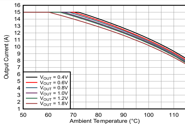
Figure 9-34. Safe Operating Area TPSM8287A12BBM V_{IN} = 3.3V
