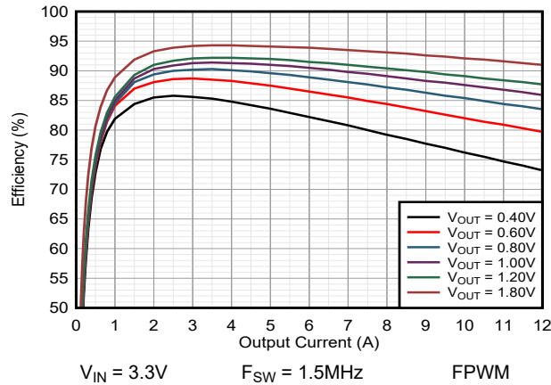
Figure 9-4. Efficiency TPSM8287A12BAM
