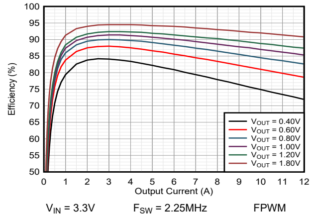
Figure 9-5. Efficiency TPSM8287A12BBM
