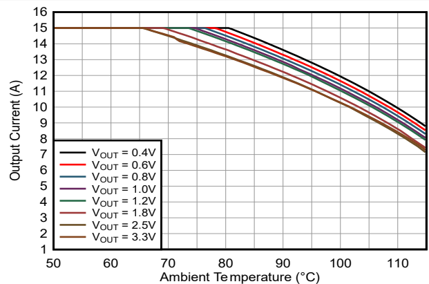
Figure 9-35. Safe Operating Area TPSM8287A12BBM V_{IN} = 5.0V
