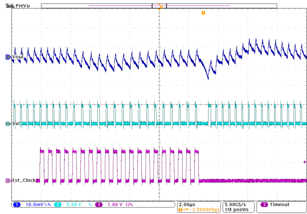
Figure 9-26. Adding and Removing an External Clock
