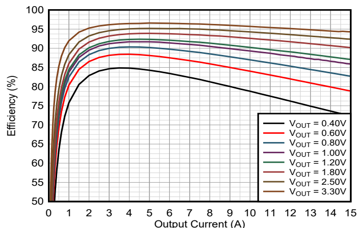
Efficiency TPSM8287A15BAM (VIN = 5.0V; FPWM)
