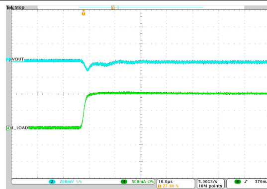
Figure 8-38. PSM-to-PWM Transition
