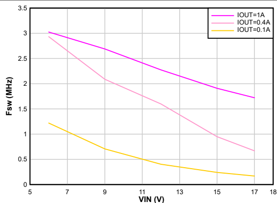
Auto PFM/PWM F_{sw} = 2.5 \text{ MHz} Figure 8-21. Switching Frequency vs Input Voltage V_{OUT} = 3.3 \text{ V}
