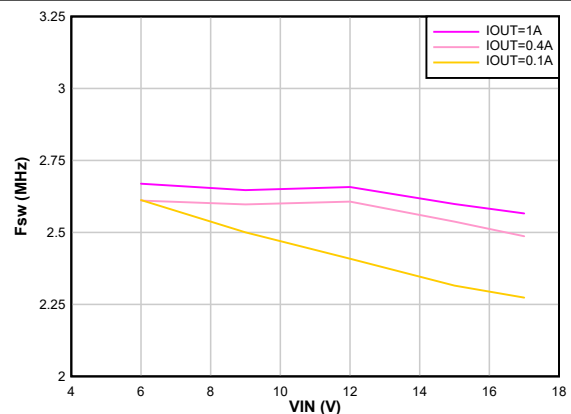
FPWM F_{sw} = 2.5 \text{ MHz} Figure 8-22. Switching Frequency vs Input Voltage V_{OUT} = 3.3 \text{ V}
