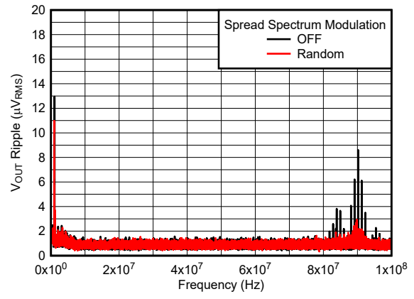
12 V to 1.8 V, 1 A 2.2 \mu\text{H} , 1 MHz First and second L-C BW = 10 kHz Figure 6-8. V_{OUT} Ripple FFT After the Second L-C Filter
