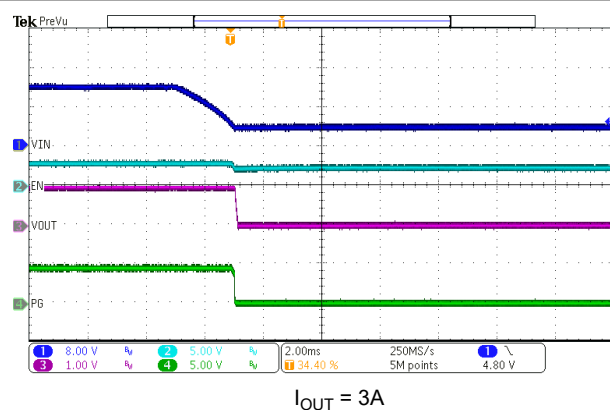
Figure 7-14. VIN Shutdown
