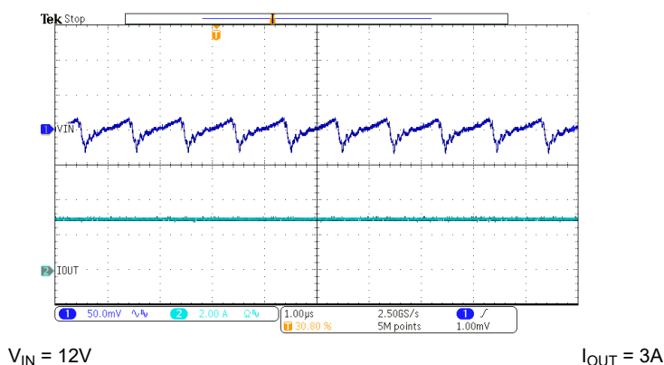
V_{IN} = 12V I_{OUT} = 3A Figure 7-18. Input Ripple – 3A Load
