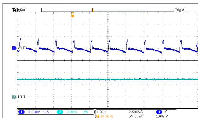
V_{IN} = 12V I_{OUT} = 3A Figure 7-16. Output Ripple – 3A Load
