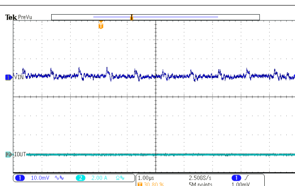
V_{IN} = 12V I_{OUT} = 0A Figure 7-17. Input Ripple – No Load
