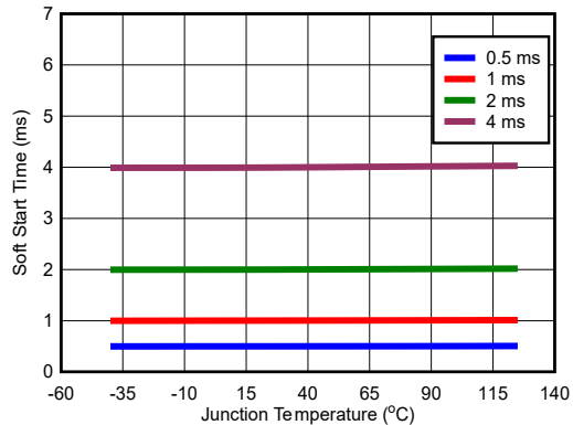
Figure 5-11. Soft Start
