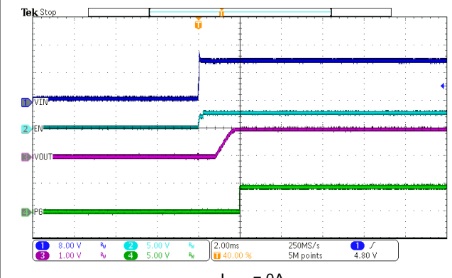
I_{OUT} = 0A Figure 7-13. VIN Start-Up
