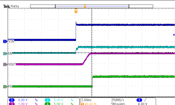
V_{IN} = 12V I_{OUT} = 8A Figure 7-11. EN Start-Up – With Load
