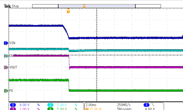
I_{OUT} = 8A Figure 7-14. VIN Shutdown
