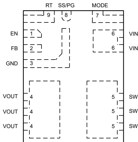
Figure 4-1. 9-Pin RCJ QFN-FCMOD, 3.3mm × 4.5mm Package (Top View)
