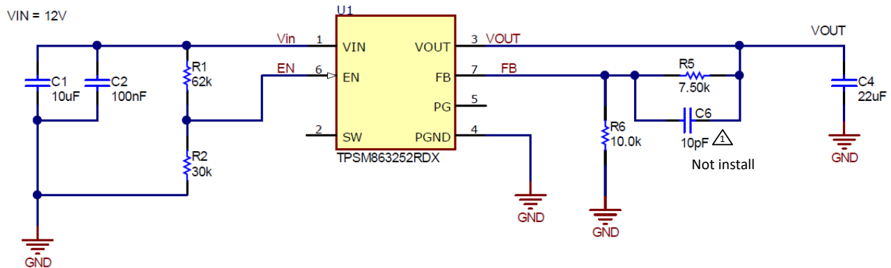
Figure 8-1. Schematic
