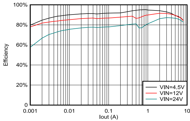
Figure 5-27. TPSM86837 Efficiency, V_{OUT} = 3.3V , F_{sw} = 1200kHz
