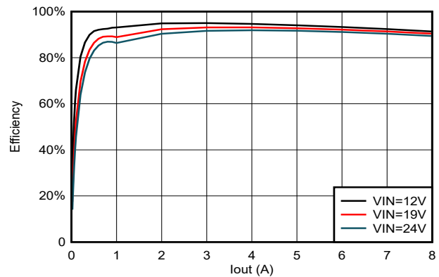
Figure 5-30. TPSM86838 Efficiency, V_{OUT} = 5V , F_{sw} = 1200kHz
