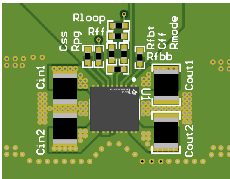
Figure 7-18. TPSM8683x Layout
