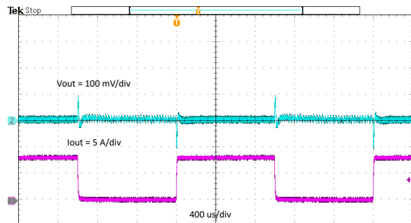
Figure 7-16. TPSM86837 Transient Response 0A to 8A
