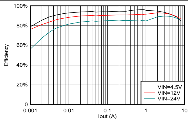
Figure 5-21. TPSM86837 Efficiency, V_{OUT} = 3.3V , F_{sw} = 800kHz
