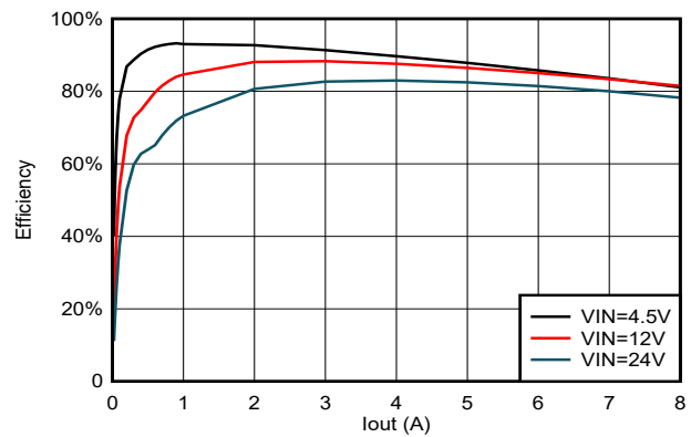
Figure 5-26. TPSM86838 Efficiency, V_{OUT} = 1.8V , F_{sw} = 1200kHz
