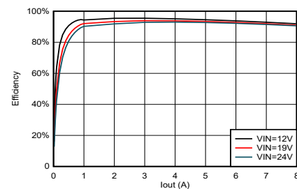
TPSM86838 Efficiency, Vout = 5V, Fsw = 800kHz
