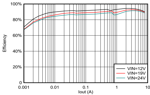
Figure 5-29. TPSM86837 Efficiency, V_{OUT} = 5V , F_{sw} = 1200kHz
