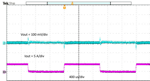
Figure 7-14. TPSM86837 Transient Response 0A to 4A
