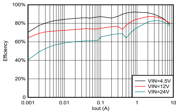
Figure 5-25. TPSM86837 Efficiency, V_{OUT} = 1.8V , F_{sw} = 1200kHz
