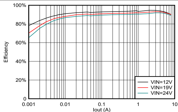
Figure 5-23. TPSM86837 Efficiency, V_{OUT} = 5V , F_{sw} = 800kHz
