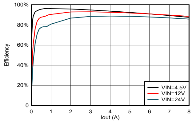
Figure 5-28. TPSM86838 Efficiency, V_{OUT} = 3.3V , F_{sw} = 1200kHz
