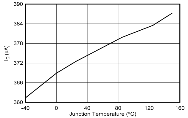
Figure 5-2. TPSM86838 Quiescent Current vs Temperature
