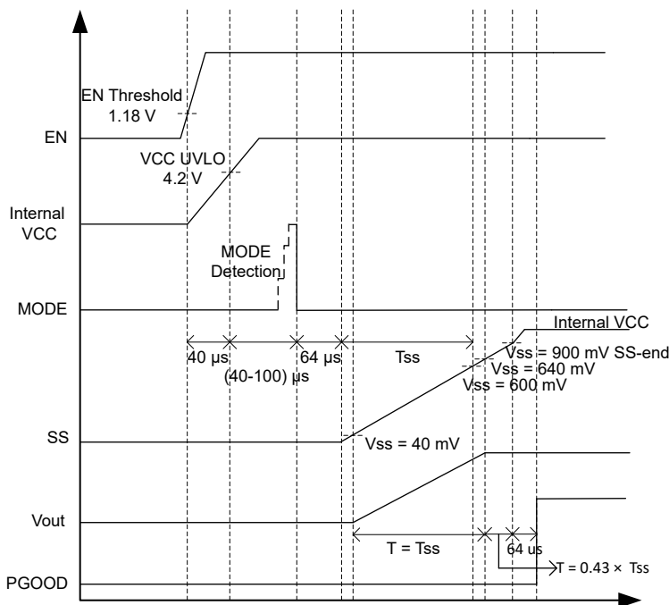
Figure 6-1. Power-Up Sequence
