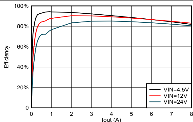
Figure 5-20. TPSM86838 Efficiency, V_{OUT} = 1.8V , F_{sw} = 800kHz
