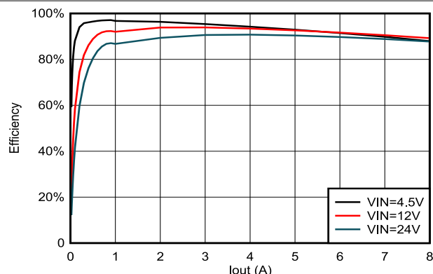
Figure 5-22. TPSM86838 Efficiency, V_{OUT} = 3.3V , F_{sw} = 800kHz
