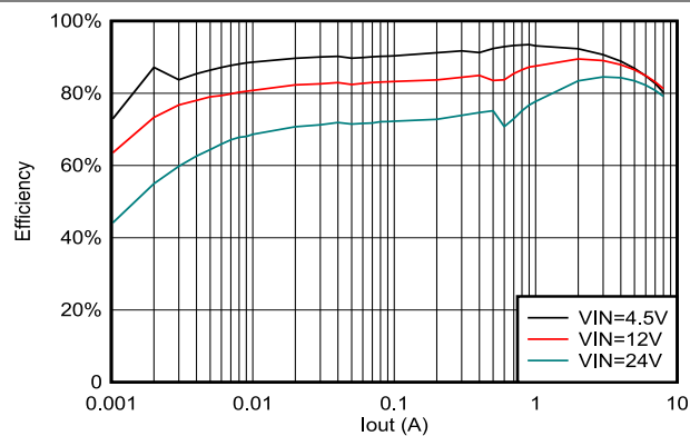
Figure 5-19. TPSM86837 Efficiency, V_{OUT} = 1.8V , F_{sw} = 800kHz
