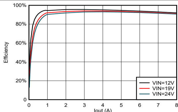
Figure 5-24. TPSM86838 Efficiency, V_{OUT} = 5V , F_{sw} = 800kHz
