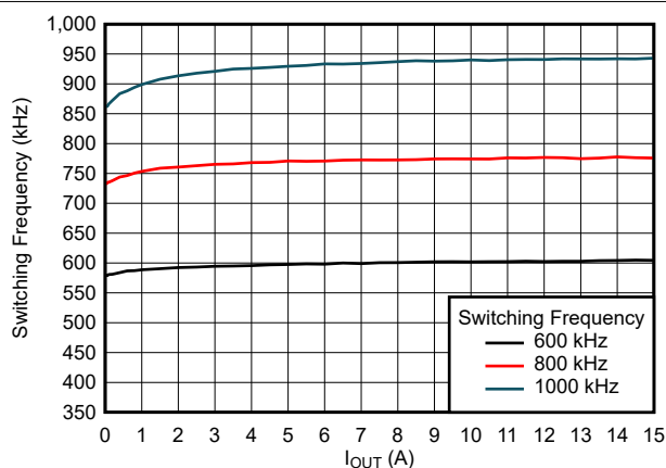
Figure 8-20. Switching Frequency
