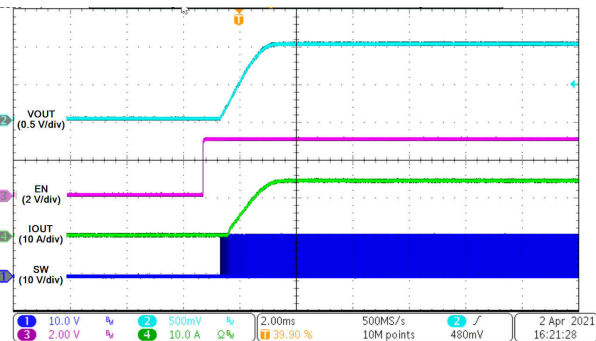
Figure 8-34. Startup Through Enable
