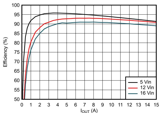
Figure 8-5. Efficiency
