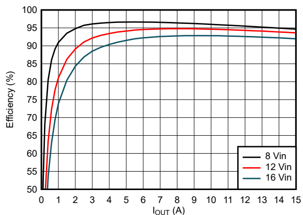
Figure 8-7. Efficiency
