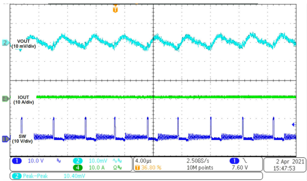
Figure 8-29. Output Voltage Ripple, V_{RIPPLE} = 10.4\text{ mV}
