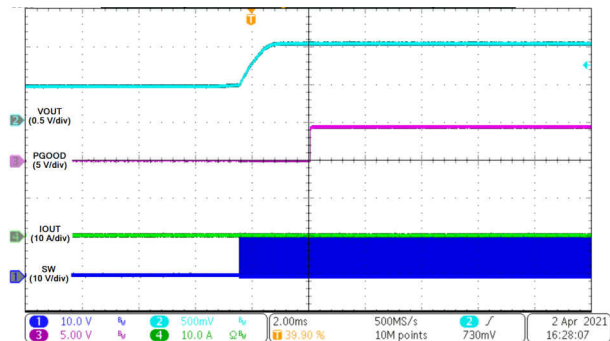
Figure 8-35. Startup Through Enable into Prebiased Load
