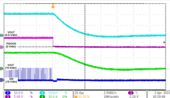
Figure 8-36. Shutdown Through Enable
