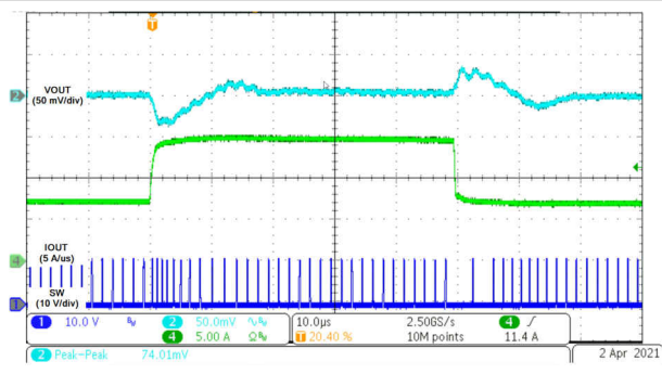
Figure 8-37. Transient Response, V PP = 74 mV
