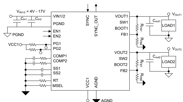
Typical Schematic
