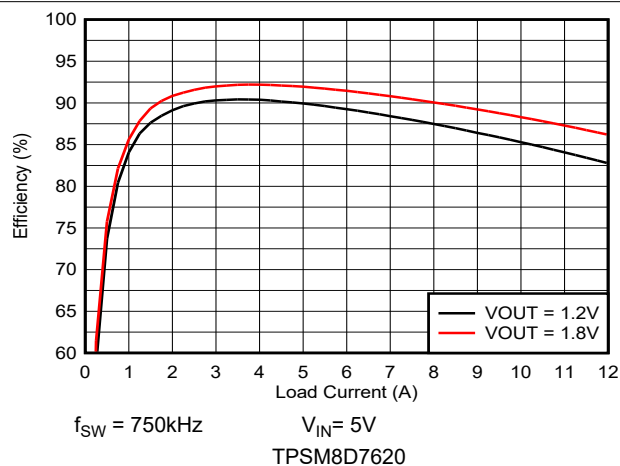
Figure 8-22. Efficiency vs Output Current
