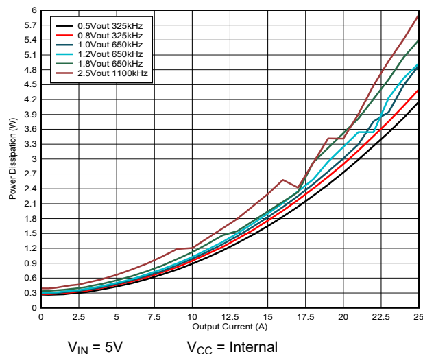
Figure 5-3. TPSM8S6B24S Power Dissipation vs Output Current
