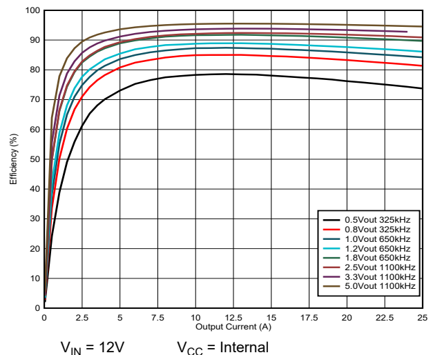
Figure 5-2. TPSM8S6B24S Efficiency vs Output Current
