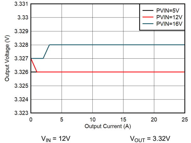
Figure 8-2. Load Regulation
