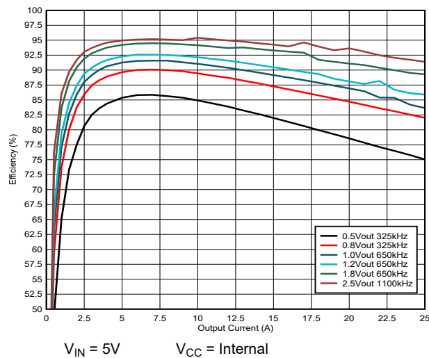
Figure 5-1. TPSM8S6B24S Efficiency vs Output Current
