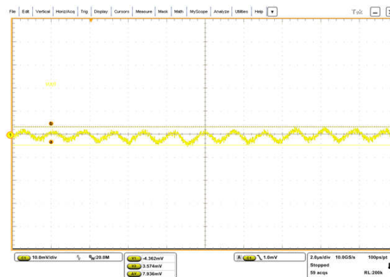
Figure 8-18. V_{OUT} Steady-State Ripple
