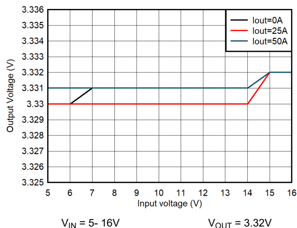
Figure 8-13. Line Regulation
