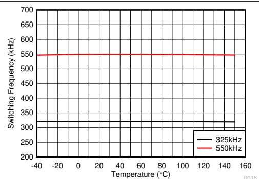
Figure 5-6. Switching Frequency vs Junction Temperature
