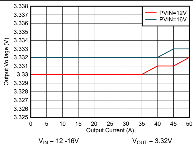
Figure 8-12. Load Regulation
