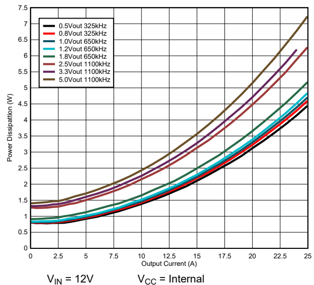
Figure 5-4. TPSM8S6B24S Power Dissipation vs Output Current
