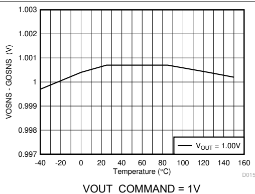
Figure 5-5. Output Voltage vs Junction Temperature
