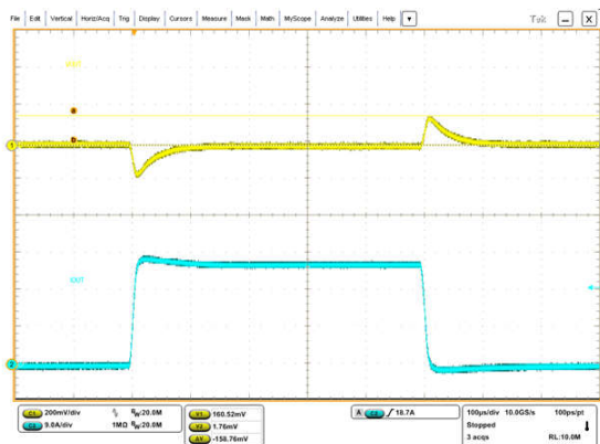
Figure 8-17. Load Transient Response
