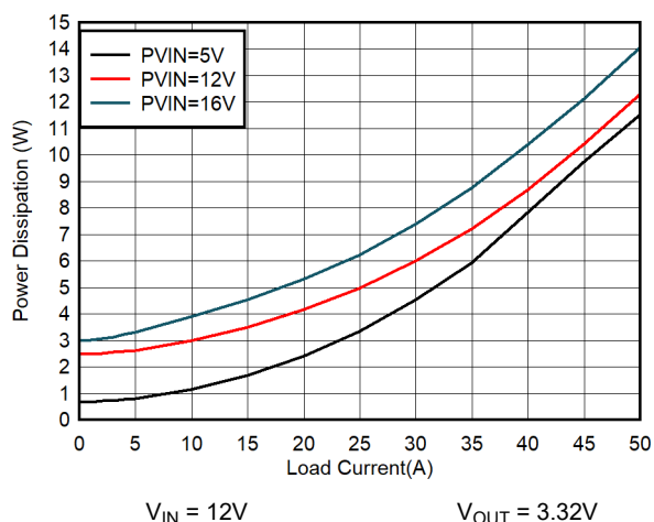
Figure 8-14. Power Dissipation
