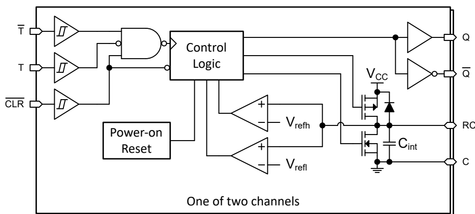
Figure 7-4. TPUL2T122A-Q1
