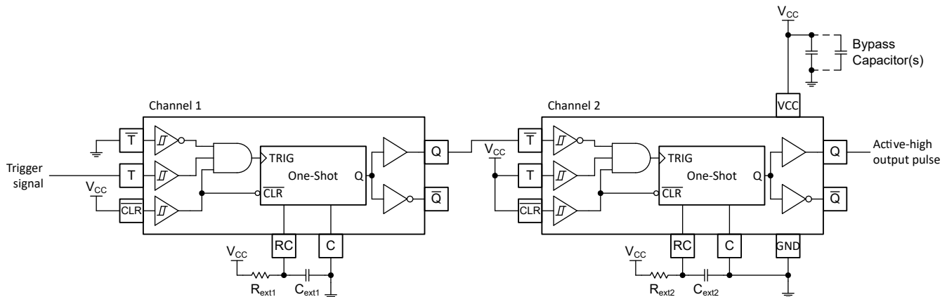
Figure 8-4. Delayed Pulse Generation Schematic Using the TPUL2T122x
