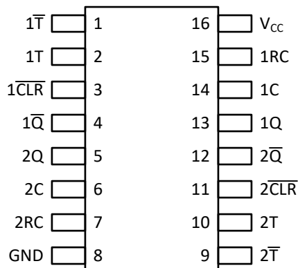
Figure 4-1. TPUL2T122 D and PW Package 16-Pin SOIC and TSSOP Top View
