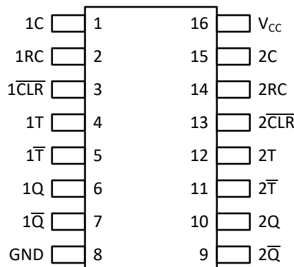
Figure 4-2. TPUL2T122A D and PW Package 16-Pin SOIC and TSSOP Top View
