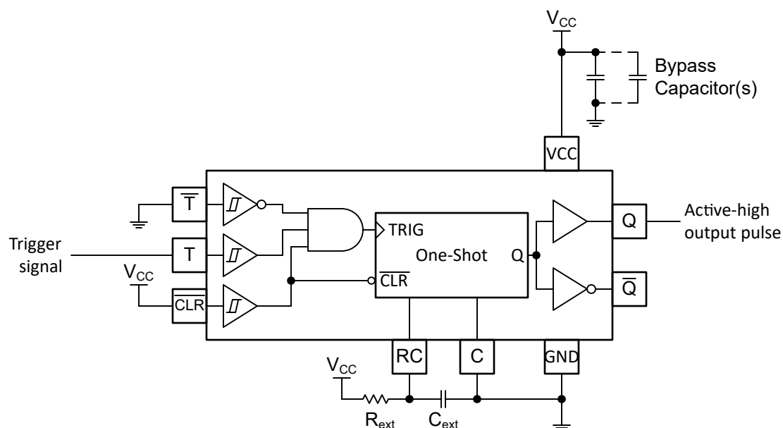
Figure 8-1. Pulse Generator Schematic Using the TPUL2T122x
