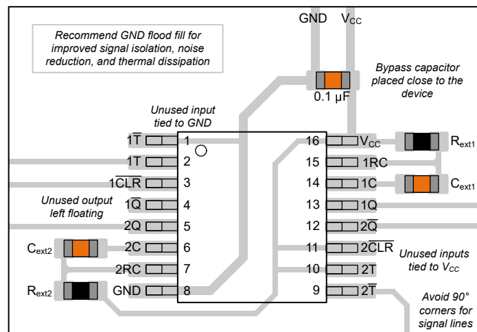
Figure 8-6. Layout Example for TPUL2T122x in the PW (TSSOP) package
