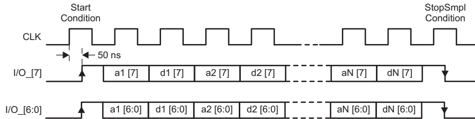
Figure 6-11. Parallel Interface Communication With Simple Stop Condition (StopSmpI)
