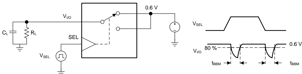
Figure 18. t_{SKEW}
