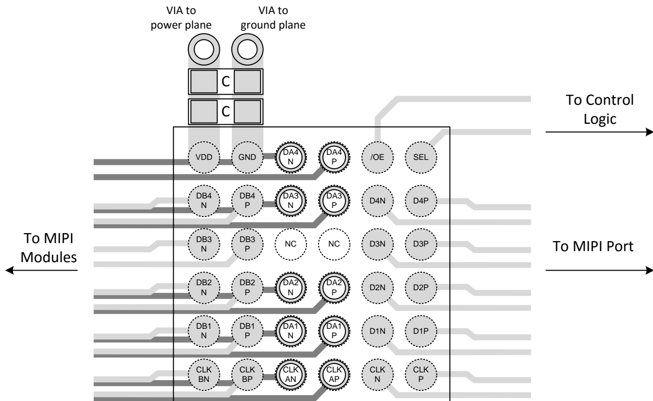
Figure 26. Layout Example
