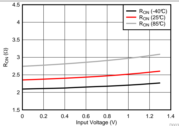
Figure 1. R_{ON} vs Input Voltage. V_{DD} = 1.65\text{ V}
