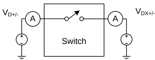
Figure 6. Off Leakage
