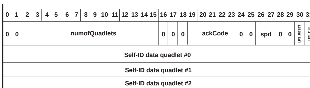
Figure 7–17. Receive Self-ID Packet Format (RXSID = 1, FULLSID = 0)
