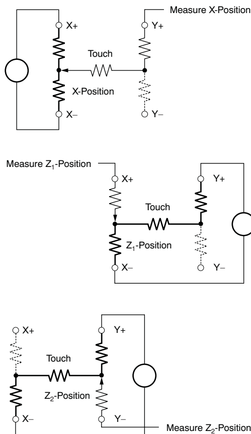
Figure 26. Pressure Measurement
