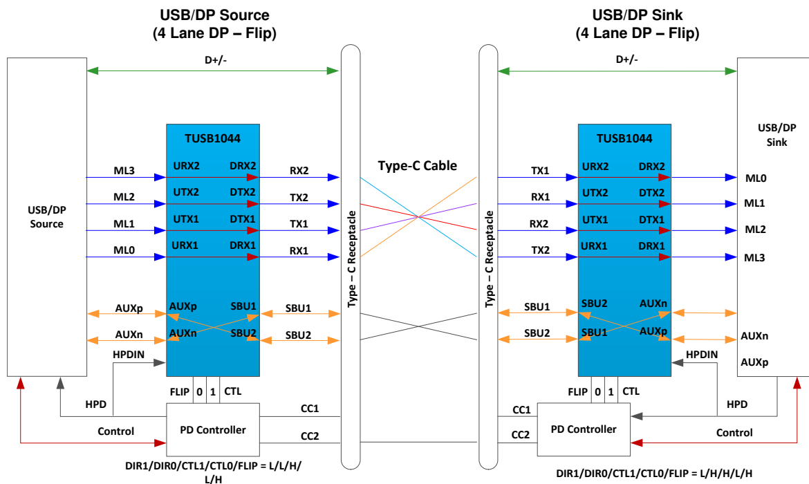
Figure 7-9. Four Lane DP – With Flip
