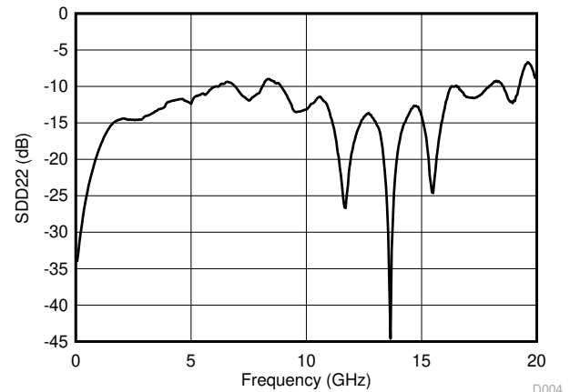
Figure 5-12. Output Return Loss Performance of the Upstream Ports
