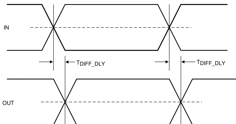
Figure 5-3. Propagation Delay
