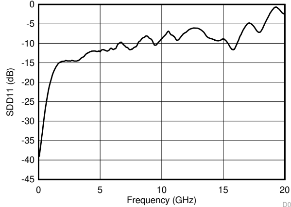
Figure 5-9. Input Return Loss Performance of the Downstream Ports
