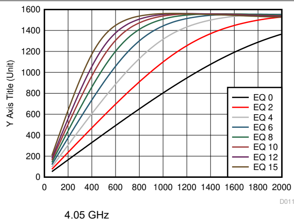
Figure 5-17. Upstream-to-Downstream Linearity Performance at 4.05 GHz
