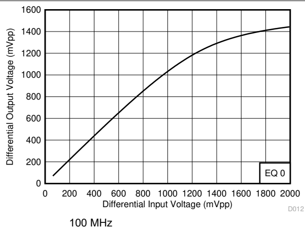
Figure 5-18. Upstream-to-Downstream Linearity Performance at 100 MHz
