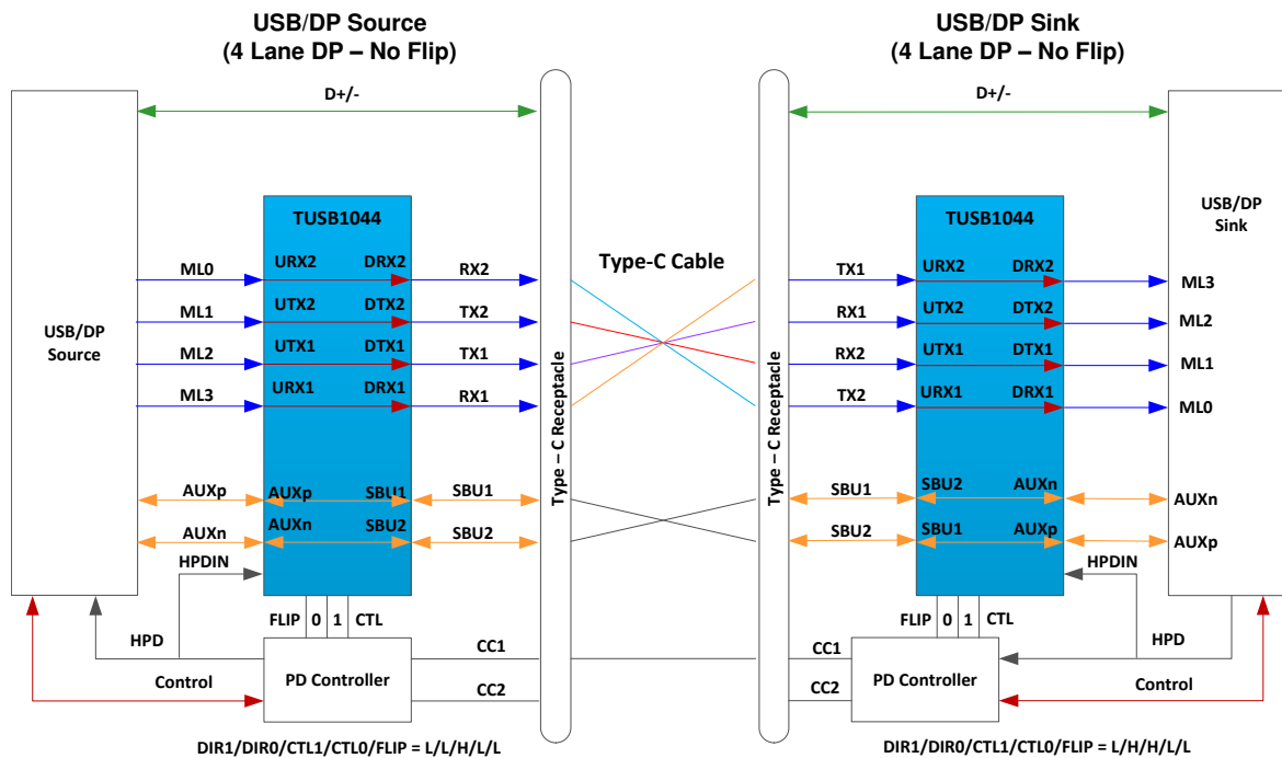
Figure 7-8. Four Lane DP – No Flip
