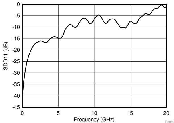
Figure 5-11. Input Return Loss Performance of the Upstream Ports
