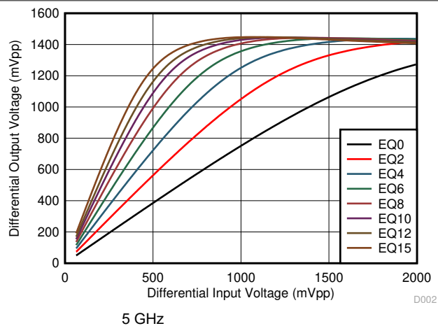
Figure 5-16. Upstream-to-Downstream Linearity Performance at 5 GHz
