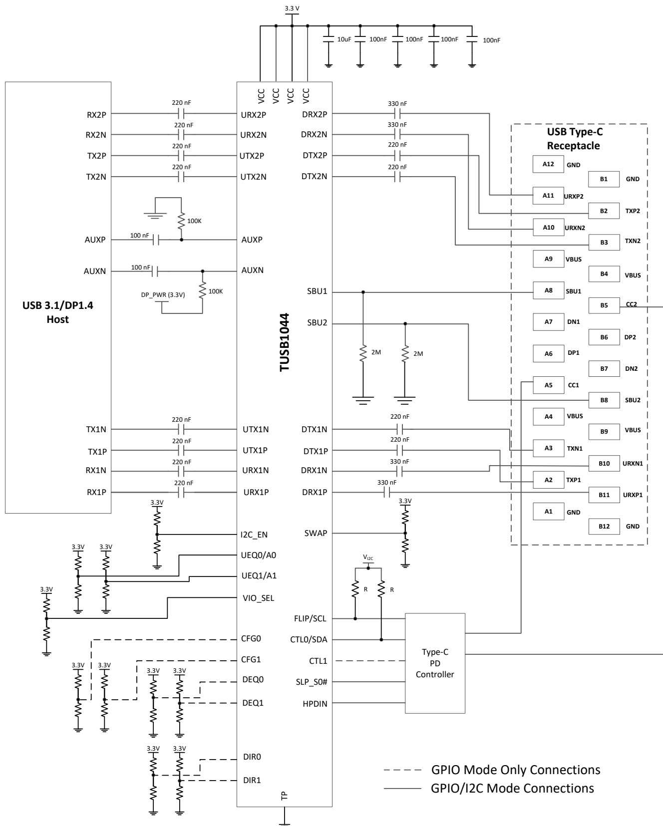
Figure 7-2. Typical Application Circuit
