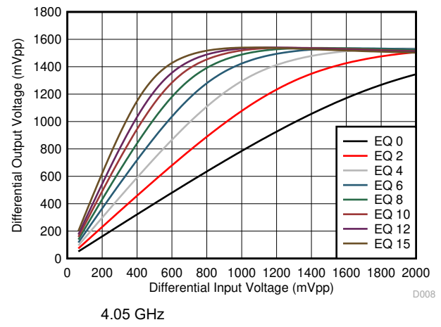
Figure 5-14. Downstream-to-Upstream Linearity Performance at 4.05 GHz
