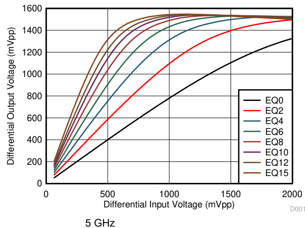
Figure 5-13. Downstream-to-Upstream Linearity Performance at 5 GHz
