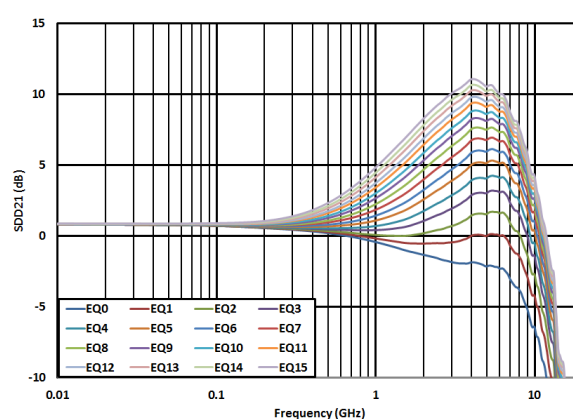
Figure 2. USB RX (DFP) EQ Settings Curves
