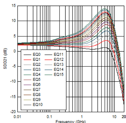
Figure 5-3. USB SSTX EQ Settings Curves
