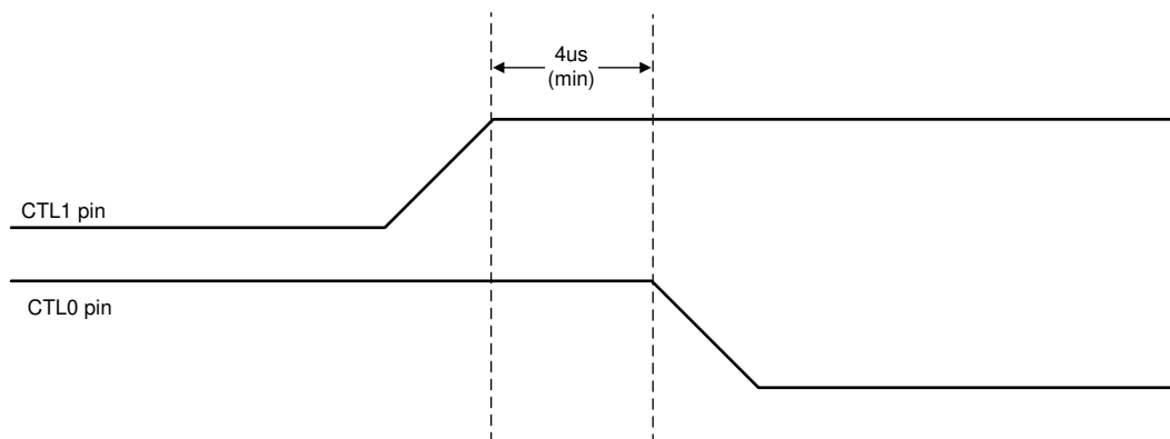
Figure 6-2. USB3.1 to 4-Lane DisplayPort in GPIO Mode
