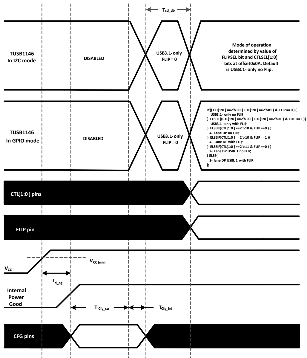
Figure 6-11. Power-On Timing
