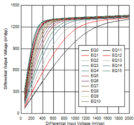
Figure 5-5. USB TX Linearity Curves at 5 GHz
