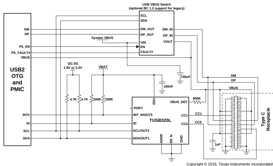
Figure 12. DRP in I²C Mode Schematic
