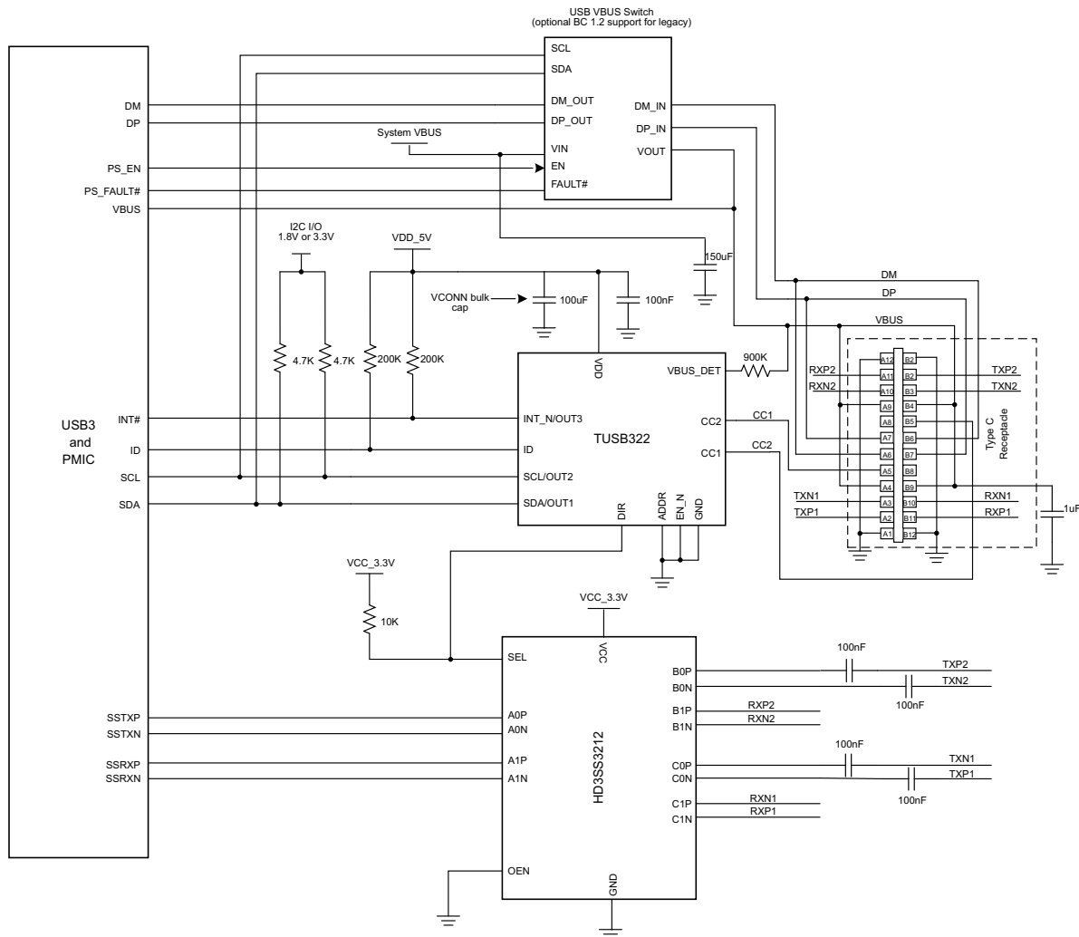
Figure 7-5. UFP in I 2 C Mode Schematic
