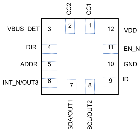
Figure 4-1. RWB Package 12-Pin X2QFN Top View
