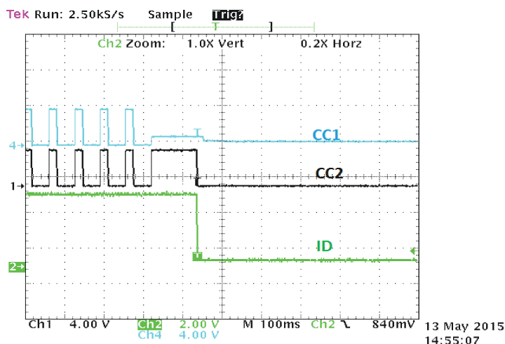
Figure 7-2. Application Curve for DRP in I 2 C Mode
