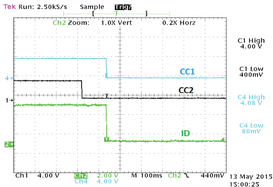
Figure 7-4. Application Curve for DFP in I 2 C Mode
