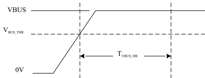
Figure 5-1. VBUS Detect and Debounce
