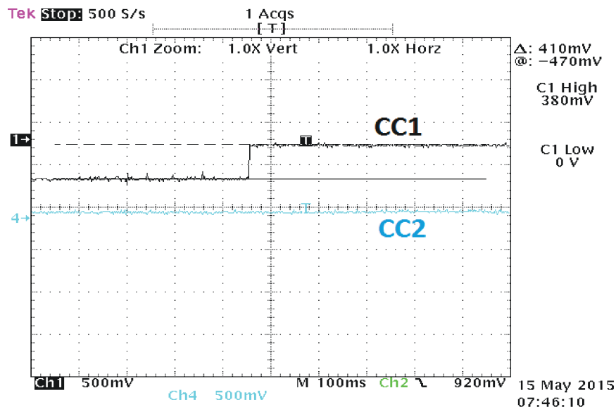
Figure 7-6. Application Curve for UFP in I 2 C Mode
