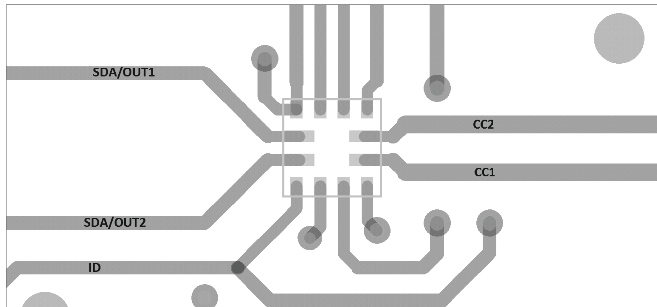
Figure 8-1. TUSB322I Layout
