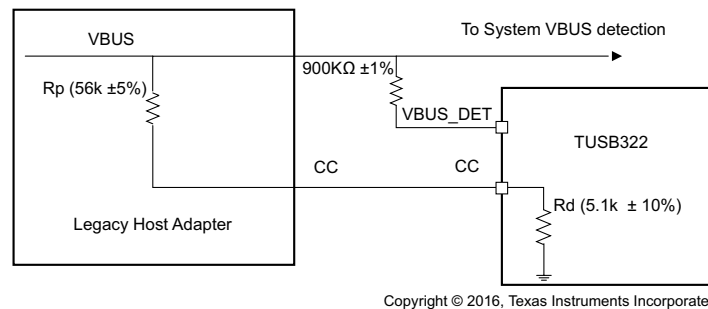
Figure 6-1. Legacy Adapter Implementation Circuit
