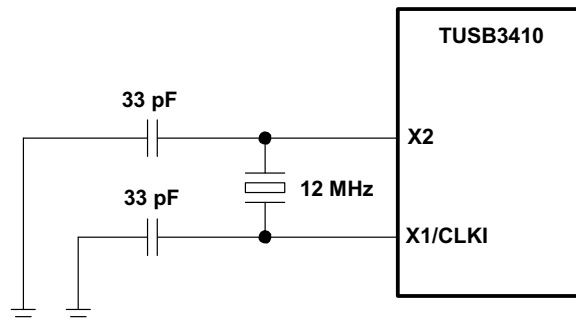
Figure 6-10. Crystal Selection
