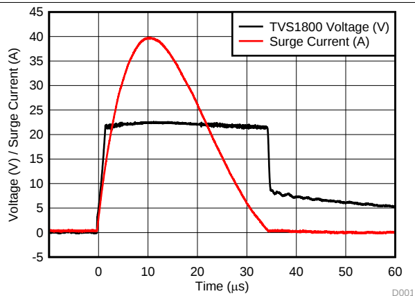
Figure 1. Surge Response at 40 A
