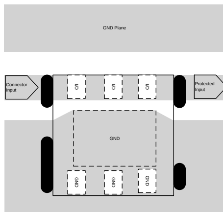
Figure 12. TVS1800 Layout
