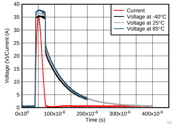
Figure 2. 8/20 μs Surge Response at 35 A Across Temperature
