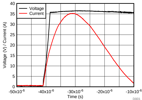
Figure 1. 8/20 μs Surge Response at 35 A
