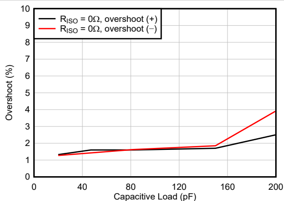
Figure 5-5. Small-Signal Overshoot vs Capacitive Load (New Die)
