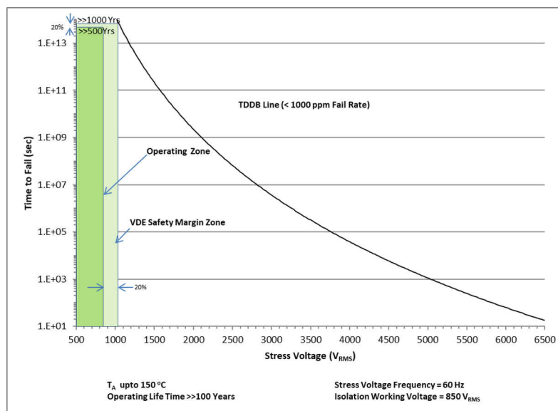
Figure 7-1. TDDB: Insulation Lifetime Projection for 850\text{ V}_{RMS} Working Voltage.
