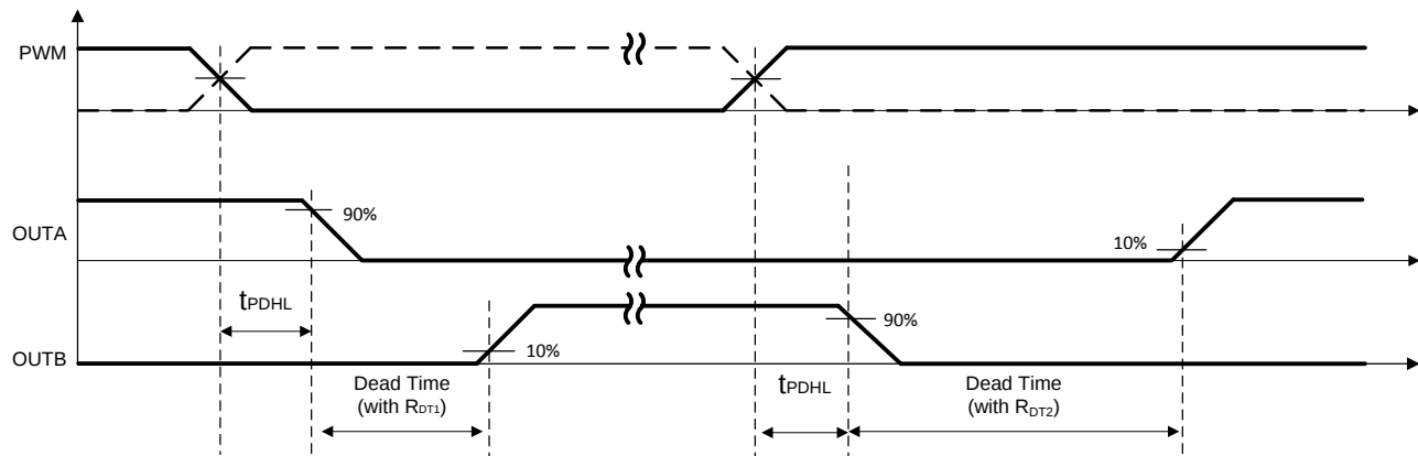
Figure 27. Dead-Time Switching Parameters
