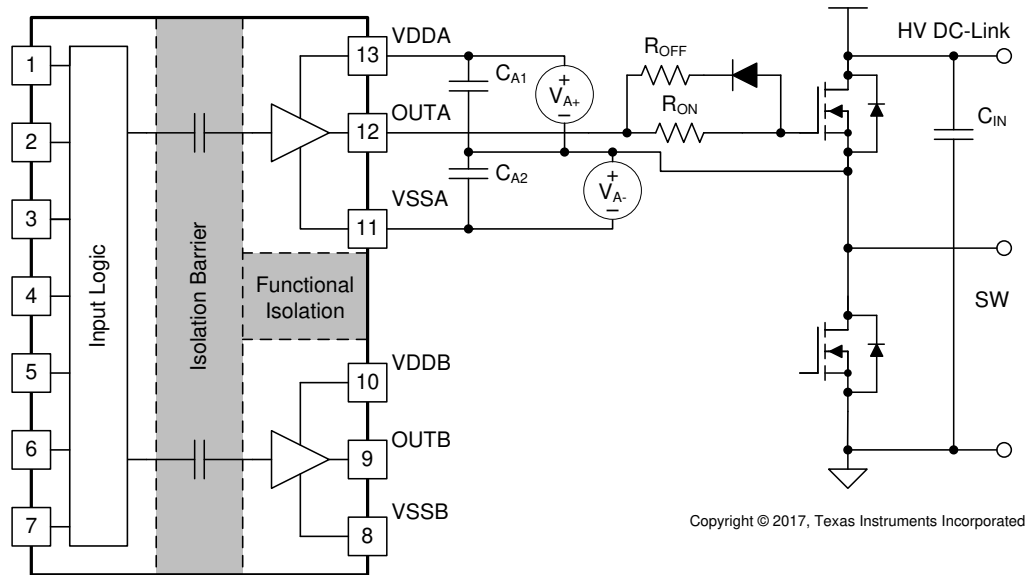
Figure 39. Negative Bias with Two Iso-Bias Power Supplies
