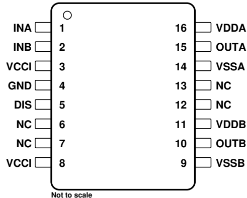
Figure 5-1. D Package 16-Pin SOIC Top View
