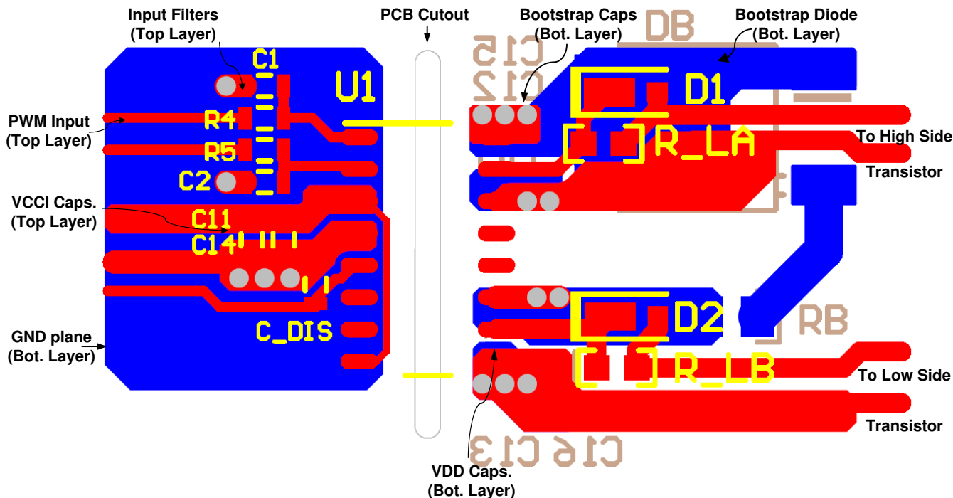
Figure 11-1. Layout Example
