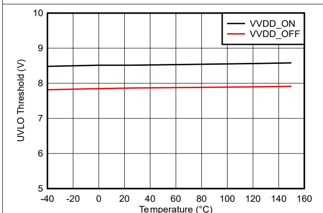
Figure 6-7. 8-V VDD UVLO Threshold Voltage
