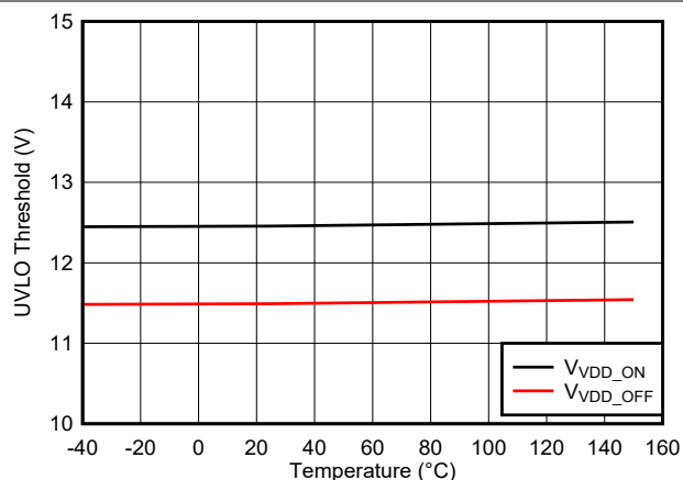
Figure 5-16. VDD 12-V UVLO Threshold vs Temperature
