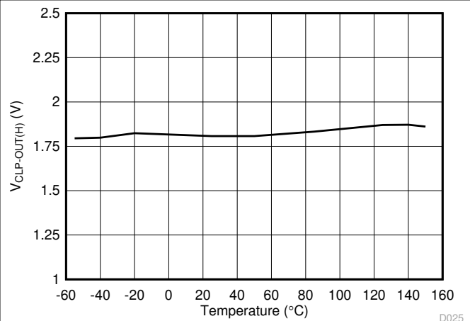
Figure 6-19. V_{CLP-OUT(H)} Short Circuit Clamping Voltage vs. Temperature
