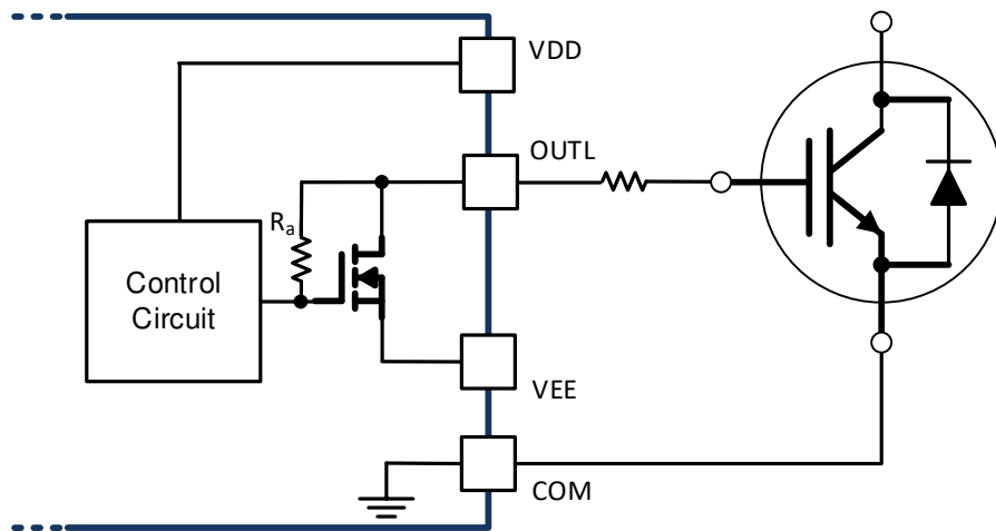
Figure 8-2. Active Pulldown
