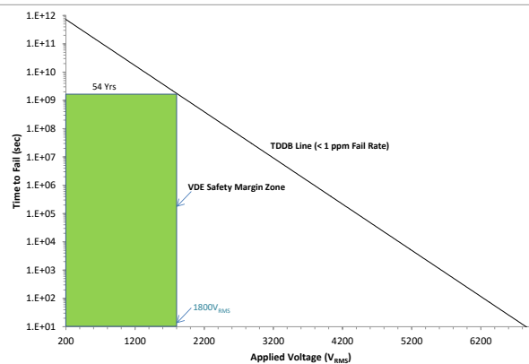
Figure 6-3. Reinforced Isolation Capacitor Life Time Projection
