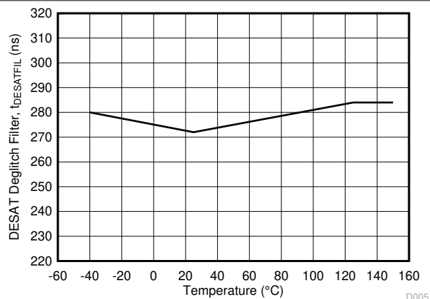
Figure 6-28. t_{\text{DESATFIL}} DESAT Deglitch Filter vs Temperature
