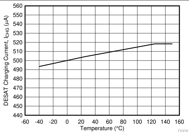
Figure 6-29. I_{\text{CHG}} DESAT Charging Current vs Temperature
