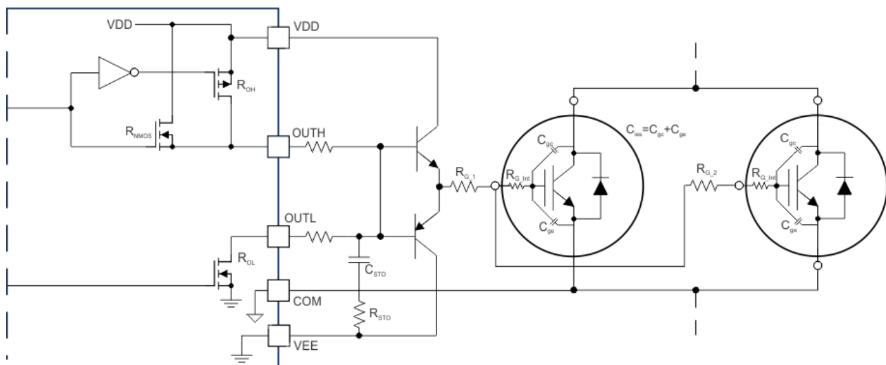
Figure 9-13. Current Buffer for Increased Drive Strength
