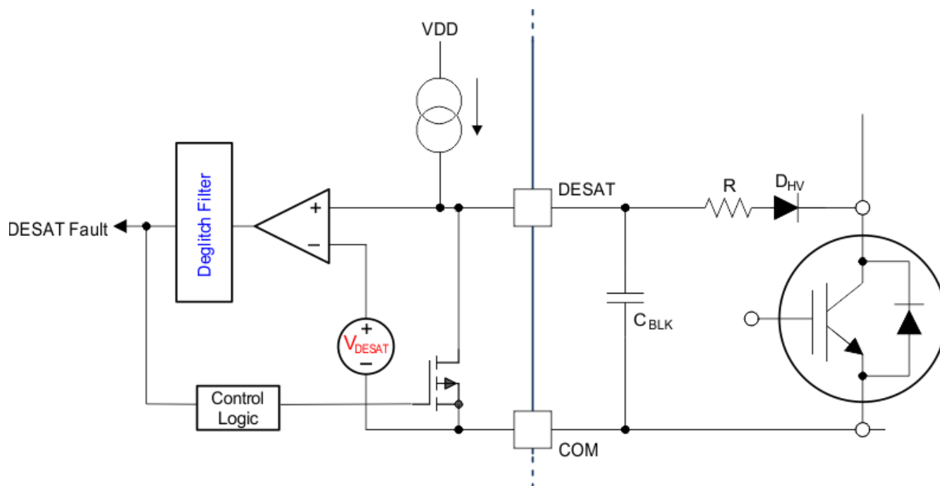
Figure 8-5. DESAT Protection
