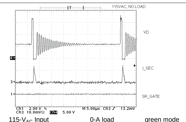
Figure 31. Secondary-Side Waveforms
