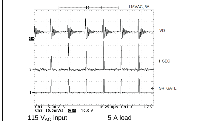
Figure 30. Secondary-Side Waveforms
