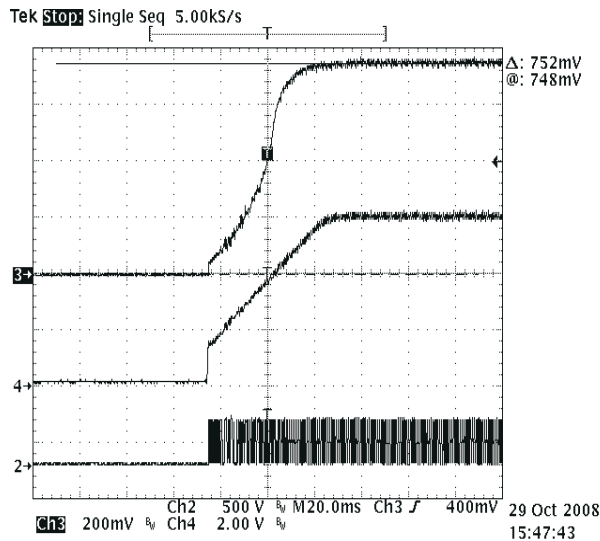
Figure 8-12. Typical Soft-Start Waveform
