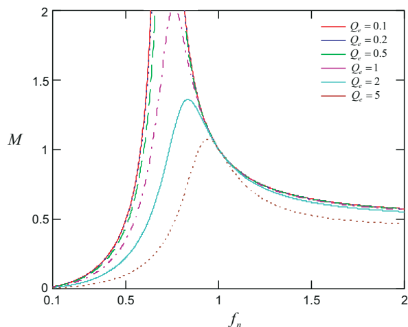
Figure 8-3. M vs f_n
