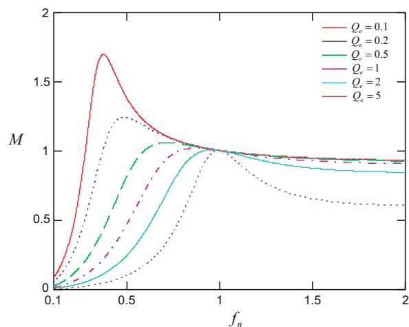
Figure 8-5. M vs f_n
