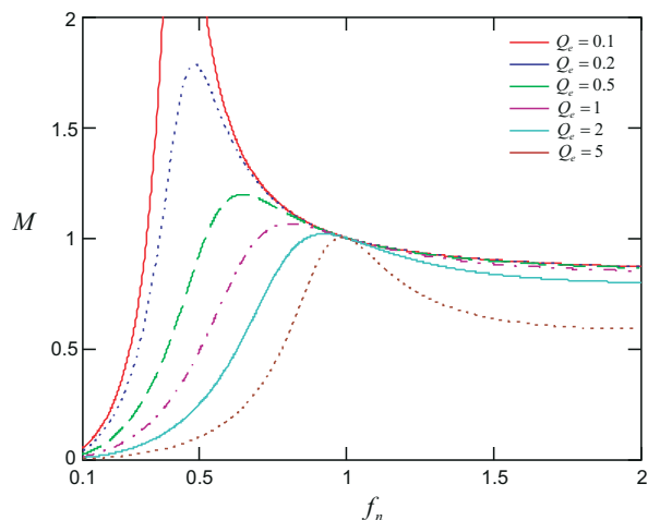
Figure 8-4. M vs f_n
