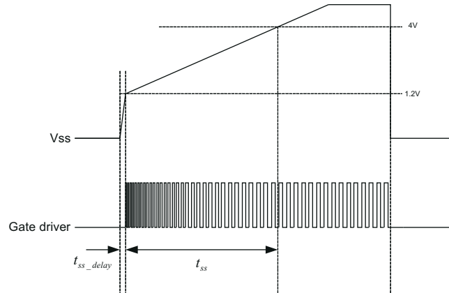
Figure 7-1. Soft-Start Sequence
