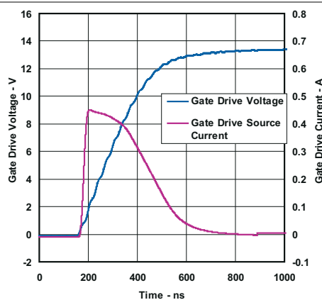
Figure 6-6. Gate Drive Rising, VCC = 15 V
