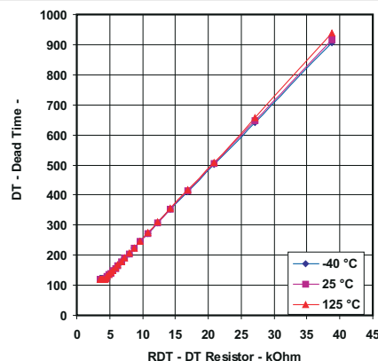
Figure 6-4. Dead Time vs DT Resistor
