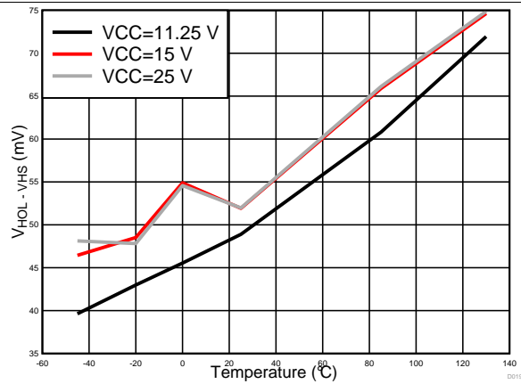
Figure 19. V_{\text{HOL}} - V_{\text{HS}} vs Temperature
