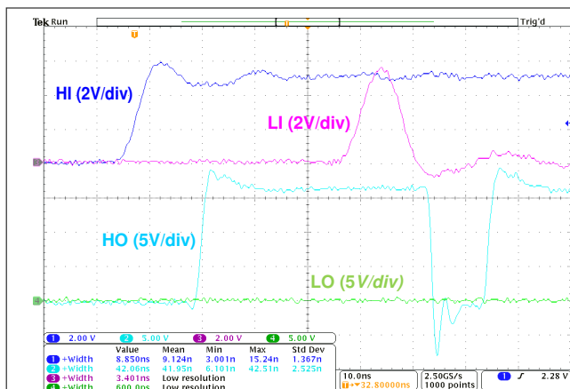
Figure 8-9. Input Shoot-through Protection or Interlock
