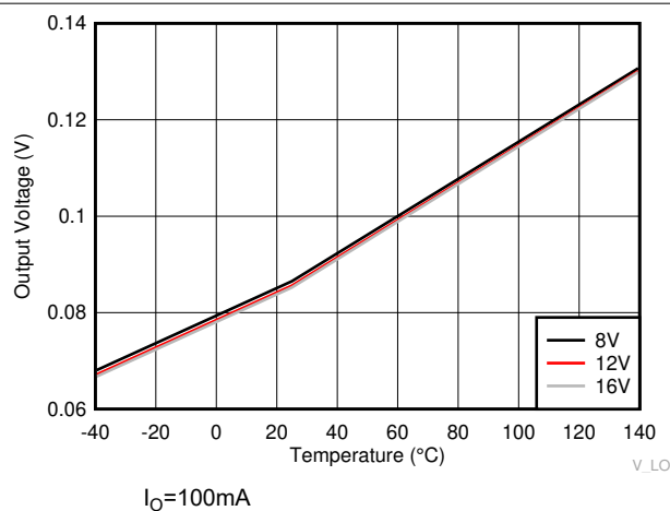
Figure 6-12. LO Low Output Voltage ( V_{LOL} )
