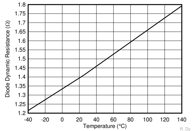
Figure 6-31. Boot Diode Dynamic Resistance
