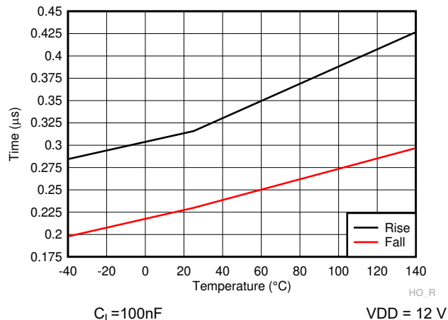
Figure 6-21. HO Rise &amp; Fall Time
