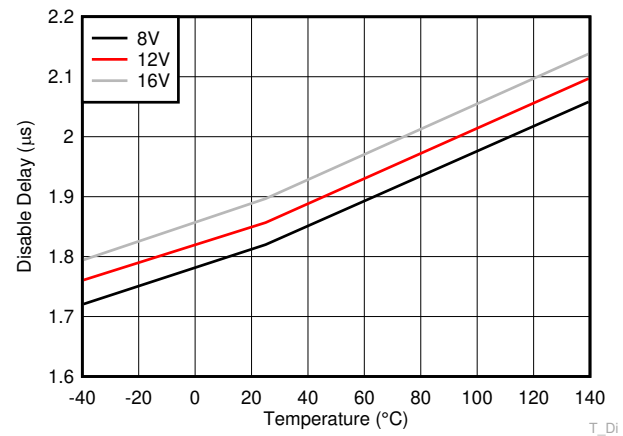
Figure 6-29. Disable Delay
