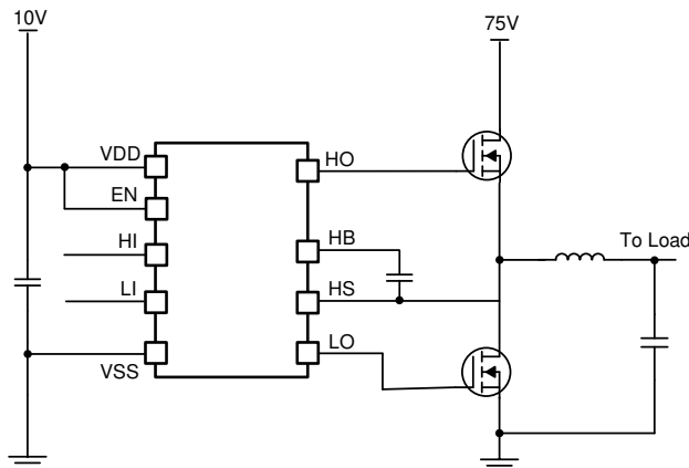
Simplified Application Diagram
