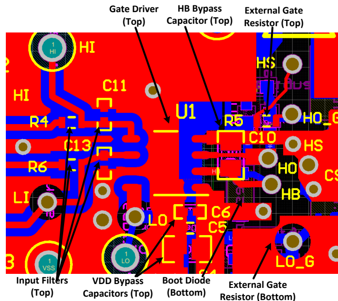
Figure 10-1. Layout Example
