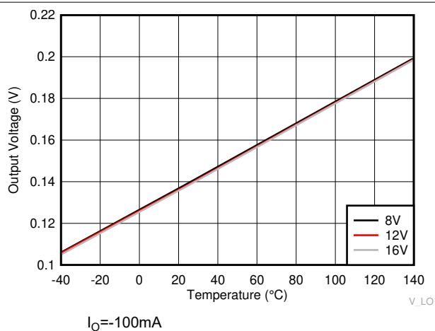
Figure 6-13. LO High Output Voltage ( V_{LOH} )
