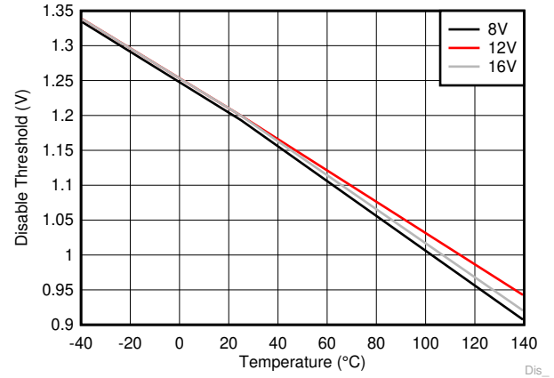
Figure 6-27. Disable Threshold
