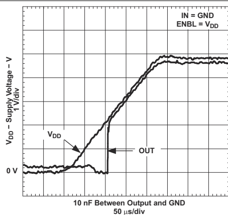
Figure 6-19. Output Behavior vs Supply Voltage (Inverting)
