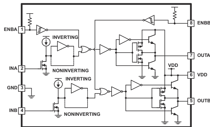
Block Diagram
