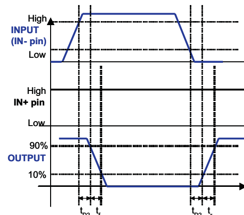
Figure 2. Inverting Configuration
