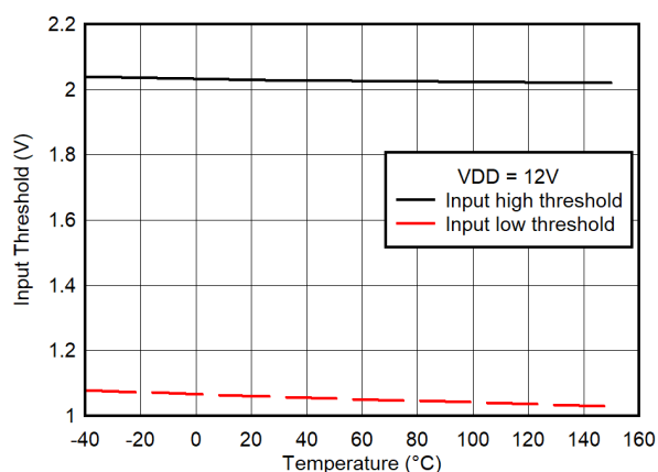
Figure 6-15. Input Threshold vs Temperature
