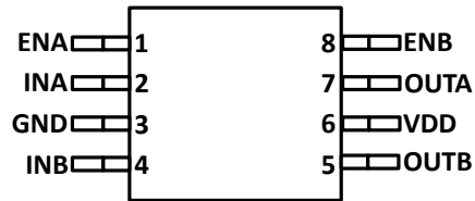
Figure 4-4. DGK Package 8-Pin VSSOP Top View
